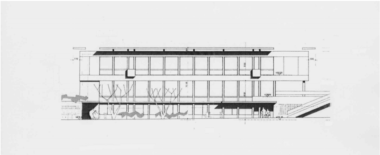
FACADE SUD
